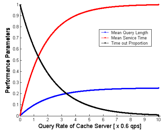
Fig. 5. Performance parameters for Scenario 4
