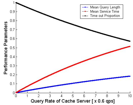
Fig. 3. Performance parameters for Scenario 2
