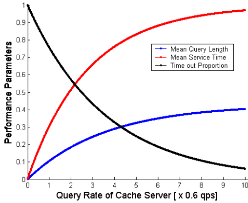
Fig. 2. Performance parameters for Scenario 1
