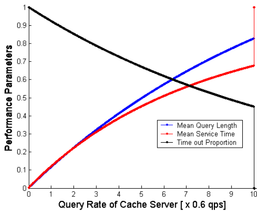
Fig. 4. Performance parameters for Scenario 3
