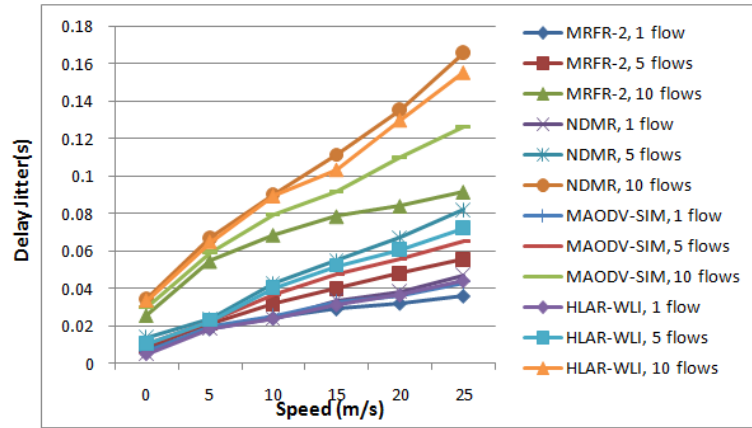
(b) Average delay jitter
