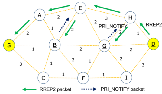
(a) Propagation of RREP2 packets.
