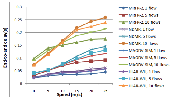
(a) Average end-to-end delay
