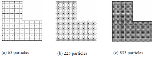
Fig. 9. Uniformly refined models
