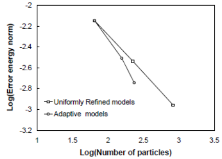
Fig. 12. Energy error norms of uniform and adaptive refinement models
