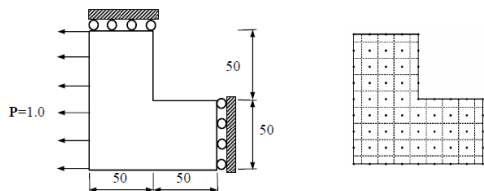
Fig. 8. L-shape domain in plane stress condition
