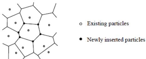
Fig. 4. Insertion of particles based on a Voronoi diagram
