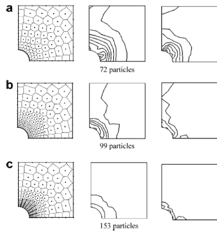
Fig. 7. a Adaptive refinement b corresponding energy error density indicator c true indicator
