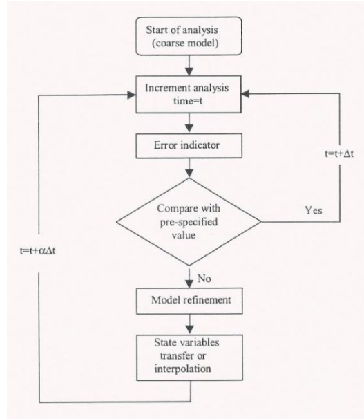
Fig. 2. Outline of progressive adaptive method
