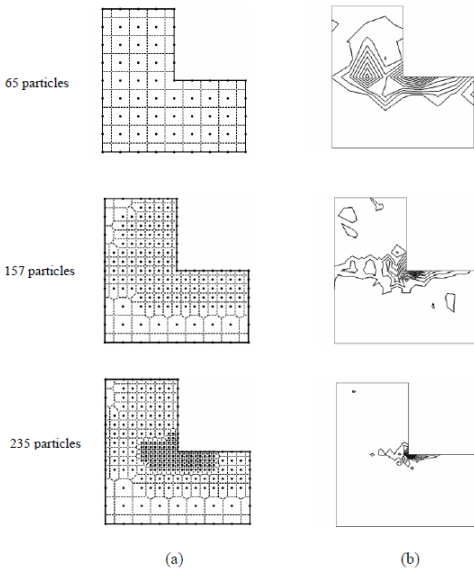
Fig. 10. (a)Adaptive refinement (b)corresponding energy error density indicator
