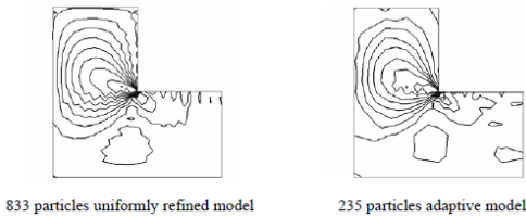
Fig. 11. Comparison of shear stress for uniform and adaptive refinement models
