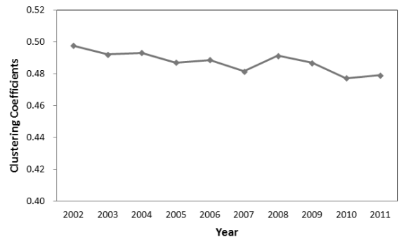
Fig. 7. Change of the clustering coefficients in the keyword networks
