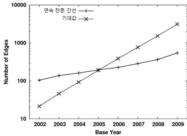
(b) The number of edges included in the skeleton
