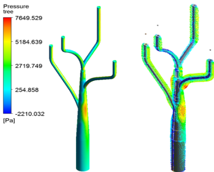
Figure 12: Interpolation result of surface pressure under 55m/s wind velocity
