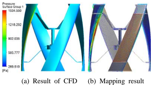
Figure 5: Interpolation result of the surface pressure under 11m/s wind velocity
