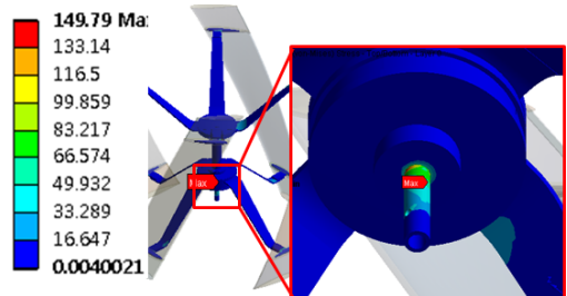
Figure 7: Equivalent stress under case 5
