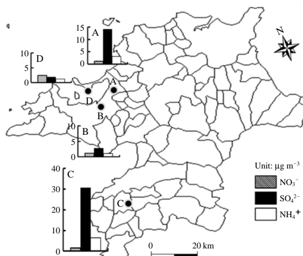
Fig. 5. Ambient concentrations of major water-soluble ions associated with \text{PM}_{2.5} collected at 4-sampling site in Fukuoka Prefecture.
