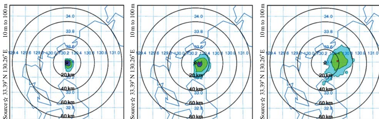
Fig. 4. Backward aerosol concentrations simulated by the NOAA ARL HYSPLIT model. The area scales mean the integrated mass concentration [ \text{mass m}^{-3} ] at 10-100 m height of site C ( 33.39^\circ \text{N} ; 130.26^\circ \text{E} ).
