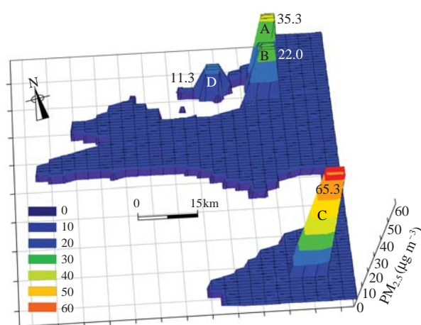
Fig. 3. 3D distribution of PM_{2.5} monitoring data at 4-sampling site.
