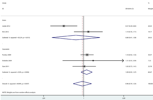
Figure 3. Forest Plots for the Association Between TLR2+1350C>T Polymorphism and Cancer Risk for Dominant Models
