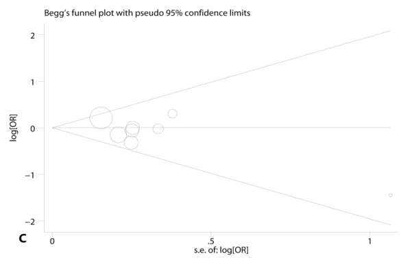
Figure 5. A: Funnel plots for the association between TLR2+597T>C polymorphism and cancer risk for dominant models. B: Funnel plots for the association between TLR2+1350C>T polymorphism and cancer risk for dominant models. C: Funnel plots for the association between TLR2 Arg753Gln polymorphism and cancer risk for dominant models
