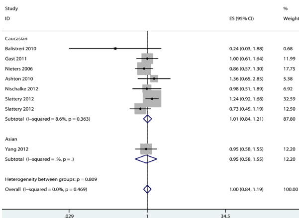
Figure 4. Forest Plots for the Association Between TLR2 Arg753Gln Polymorphism and Cancer Risk for Dominant Models
