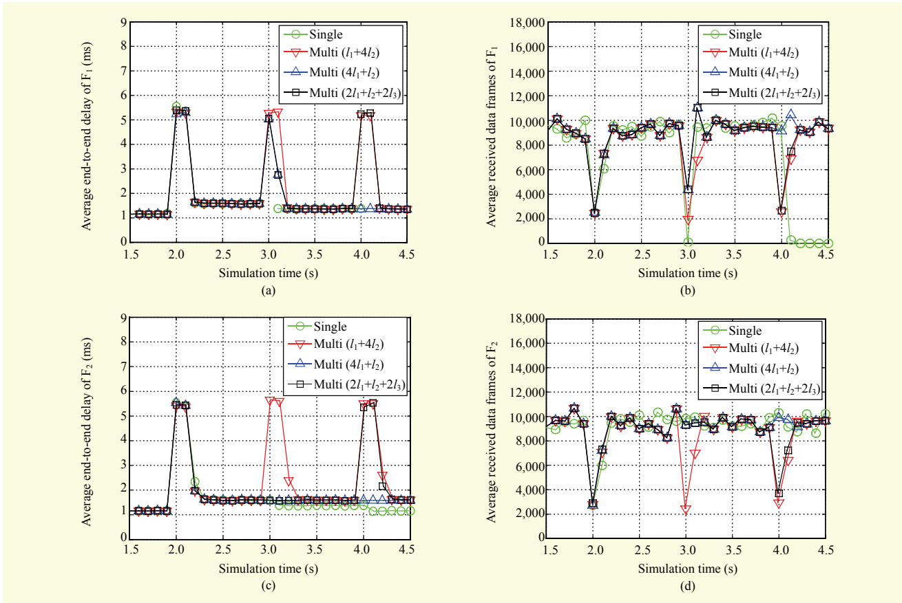
Fig. 6. Survivability performances under multiple link failures: (a) average end-to-end delay of flow F_1 , (b) average number of received data frames of flow F_1 , (c) average end-to-end delay of flow F_2 , and (d) average number of received data frames of flow F_2 .
