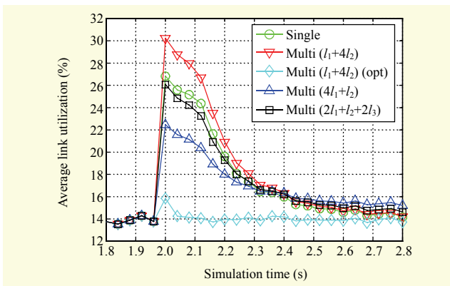
Fig. 7. Averaged link utilization under single link failures.
