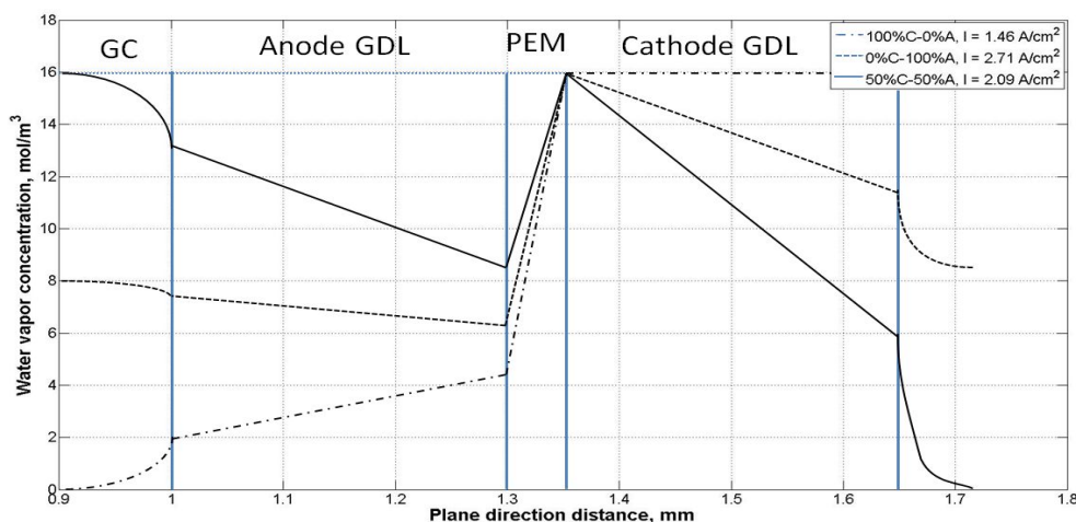
Figure 2. Water concentration variation at various important locations
