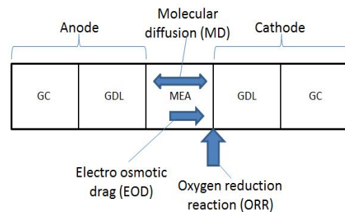
Figure 1. One dimensional control volume transfer
