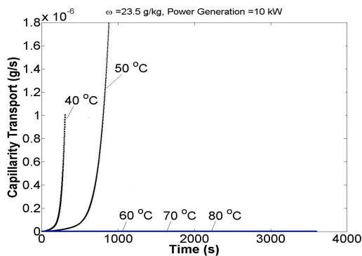
Figure 3. Capillary transport in GDL
