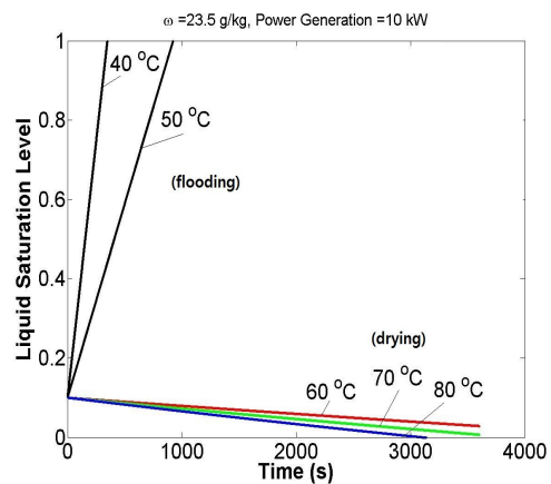
Figure 5. Liquid saturation level
