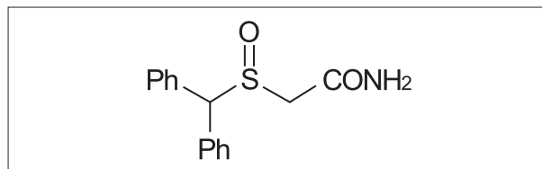
Figure 1. Modafinil structure.
