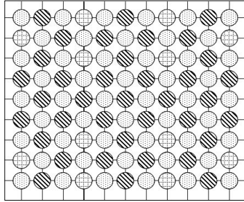
Fig. 11 Lay-out of infrared lamp(40W) distribution method ( ● infrared lamp, ▨ metal halide visible lamp, ▩ metal halide UV lamp )
