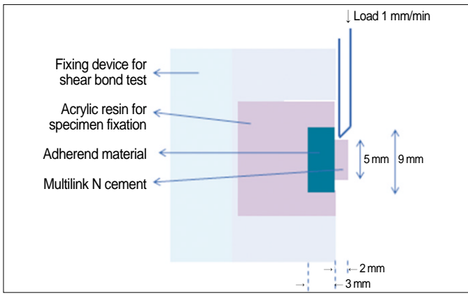
Fig. 3. Cross-sectional illustration of shear bond strength test.
