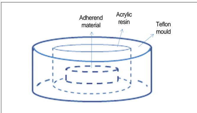
Fig. 1. Illustration of embedding specimen in the acrylic resin.
