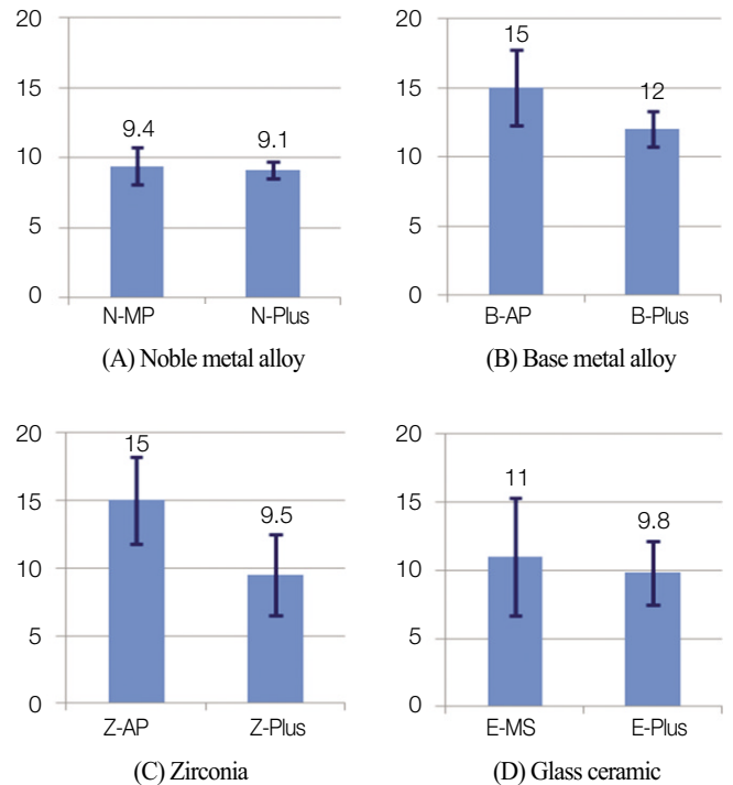
Fig. 4. Shear bond strength (MPa) between resin cement and restorative materials. *B: base metal alloy, E: glass ceramic, N: noble metal alloy, Z: zirconia, AP: Alloy primer, MP: Metal primer II, MS: Monobond-S, Plus: Monobond plus.
