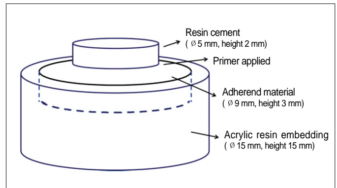
Fig. 2. Illustration of bonded specimen.
