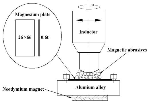
Fig. 9 Experimental setup for MAP of magnesium
