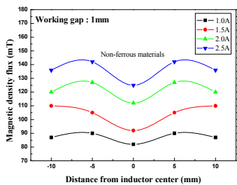
Fig. 4 Magnetic density flux of non-ferrous materials
