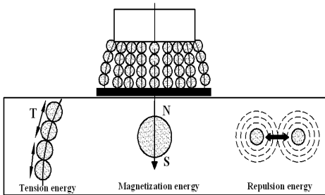
Fig. 1 Concept for micro-magnetic abrasive polishing
