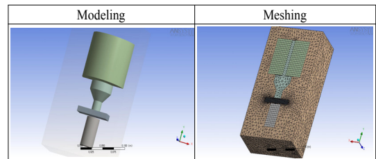
Fig. 6 Modeling and meshing with magnet
