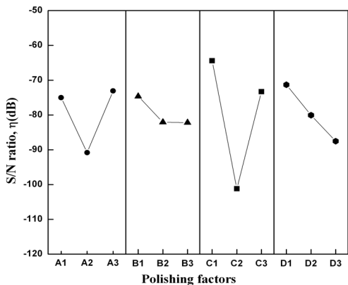
Fig. 11 Influence of factors on MAP of magnesium
