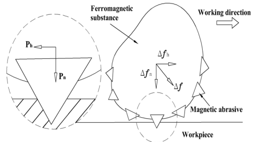
Fig. 2 Cutting force in magnetic abrasive polishing
