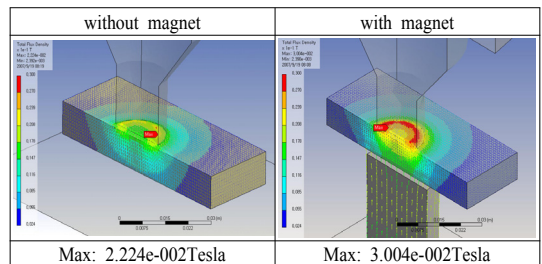
Fig. 7 Magnetic density flux compared with and without magnet
