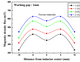
Fig. 5 Magnetic density flux of ferrous materials
