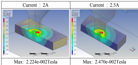
Fig. 3 Magnetic density flux for change of current
