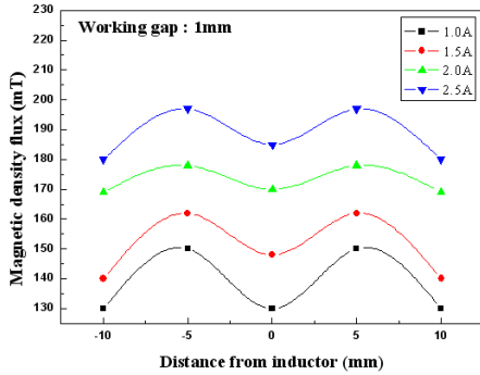
Fig. 8 Magnetic density flux on surface with permanent magnet
