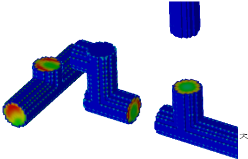
Fig. 10 Temperature distribution by improved 3D meshing.
