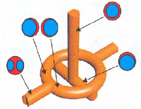
Fig. 11 Temperature distribution in MAX™
