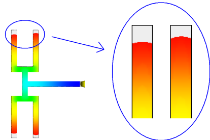
Fig. 6 Filling imbalances by improved 3D meshing
