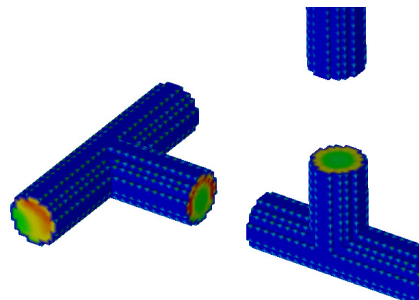
Fig. 8 Temperature distribution by improved 3D meshing.
