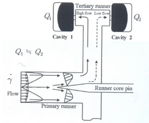
Fig. 13 Symmetrical shear distribution by RC Pin
