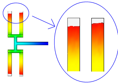
Fig. 5 Filling imbalances by conventional 3D meshing
