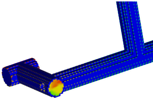
Fig. 14 Temperature distribution by improved 3D meshing.
