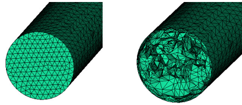
Fig. 1 Inside mesh shape by conventional 3D meshing.
