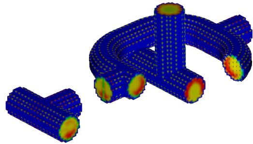
Fig. 12 Temperature distribution by improved 3D meshing.
