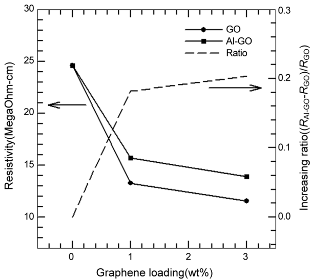
Figure 6. Electrical resistivity of DGEBA composites with graphene oxide(GO) and Al(OH) 3 functionalized graphene.
