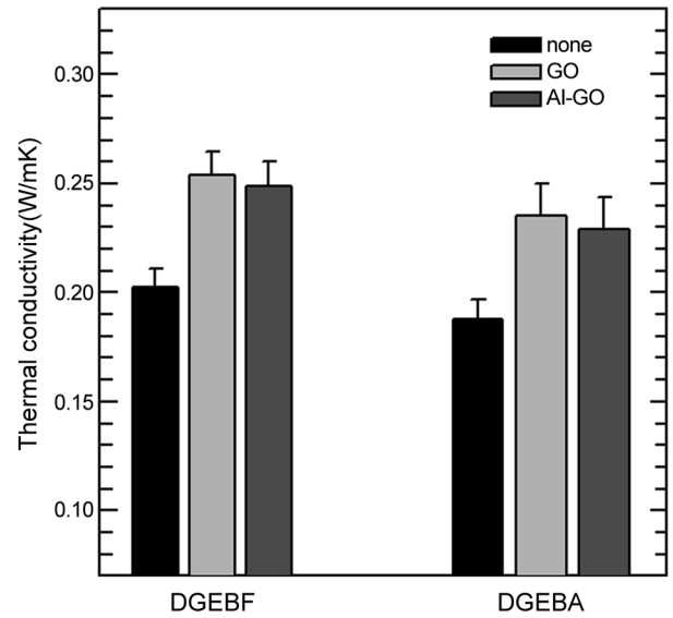
Figure 7. Thermal conductivity of DGEBF and DGEBA composites with neat epoxy, graphene oxide and Al(OH) 3 functionalized graphene.
