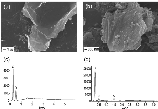
Figure 4. FE-SEM images and EDX spectra of graphene sheets (a) graphene oxide; (b) Al(OH) 3 functionalized graphene composite; (c) EDX of graphene oxide; (d) EDX of Al(OH) 3 functionalized graphene.
