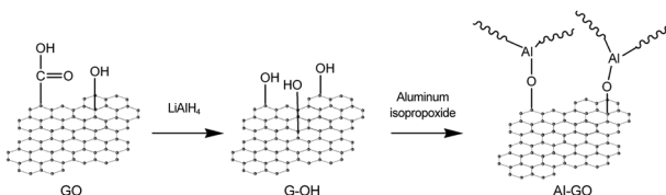
Figure 1. Preparation of modified graphene composites with aluminum isopropoxide (AIIP).
