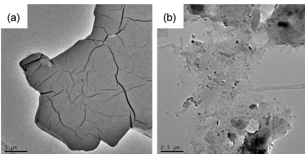
Figure 5. FE-TEM images of the graphene layers, (a) graphene oxide; (b) Al(OH) 3 functionalized graphene.
