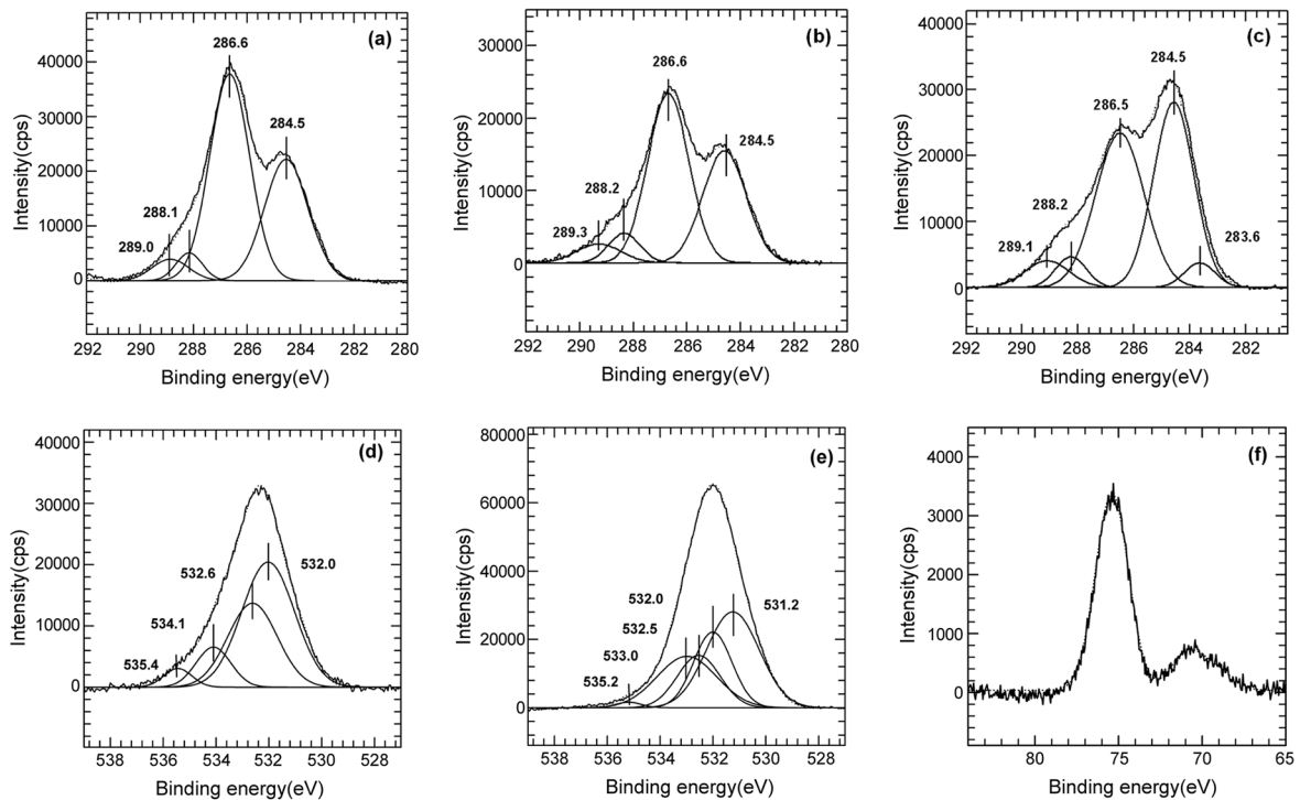
Figure 3. C 1s X-ray photoelectron spectra of (a) graphene oxide; (b) carboxylic acid reduced graphene; (c) Al(OH) 3 functionalized graphene composite; O 1s spectra of (d) carboxylic acid reduced graphene; (e) Al(OH) 3 functionalized graphene composite; Al 2p spectrum of (f) Al(OH) 3 functionalized graphene.
