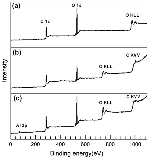
Figure 2. X-ray photoelectron spectra survey scans of (a) graphene oxide; (b) carboxylic acid reduced graphene; (c) Al(OH) 3 functionalized graphene.
