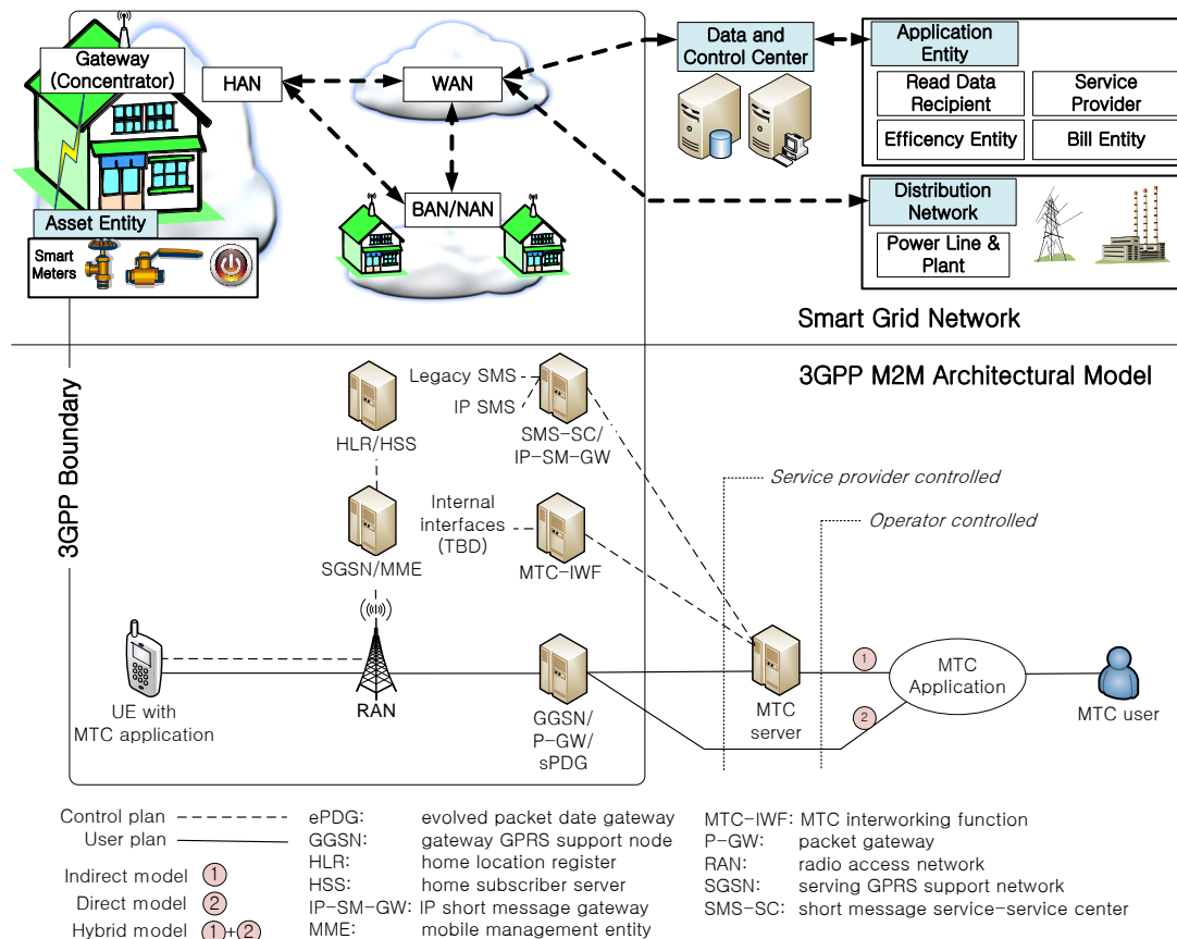
Fig. 1. Relation between smart grid network and 3GPP M2M architectural model
