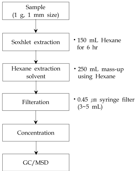
Fig. 1. Flowchart of analytical method for phthalate contents in school supplies.
