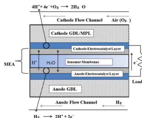
Fig. 1. Schematic cross-section of a PEM single cell.
