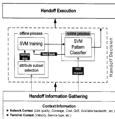
Fig. 4. Block diagram of the proposed SVM-based VHO decision system
