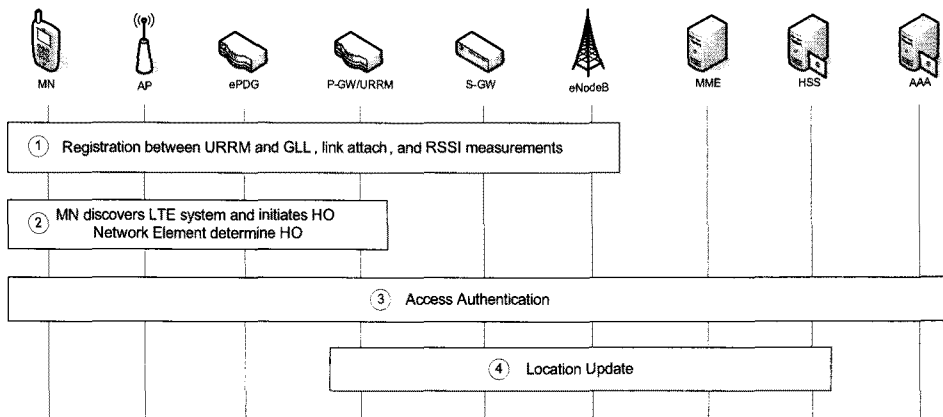
Fig. 3. A brief VHO Procedure from WLAN to LTE
