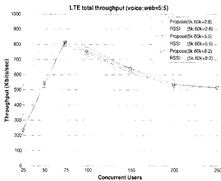
Fig. 6. LTE total throughput
