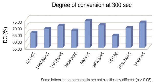
Figure 6. Degree of conversion at 300 seconds of irradiation. L, low concentration; M, medium concentration; H, high concentration.
