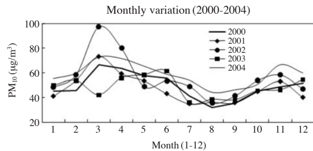
Fig. 2. Annual variations of observed PM_{10} concentrations for recent years in Busan.
