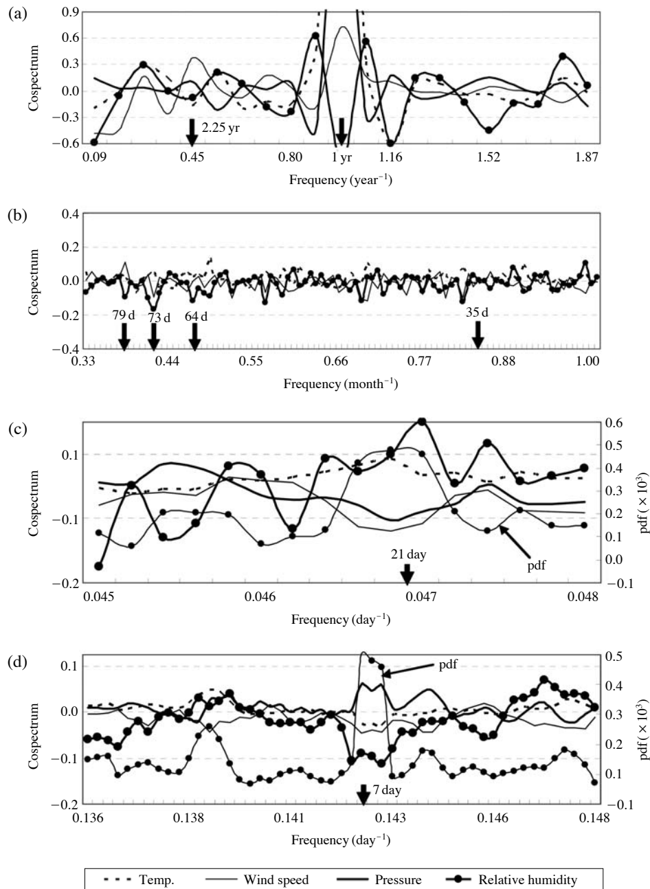
Fig. 4. Cosppectrum between PM_{10} time series and meteorological parameters (wind speed, temperature, and surface pressure in the Busan metropolitan area).
