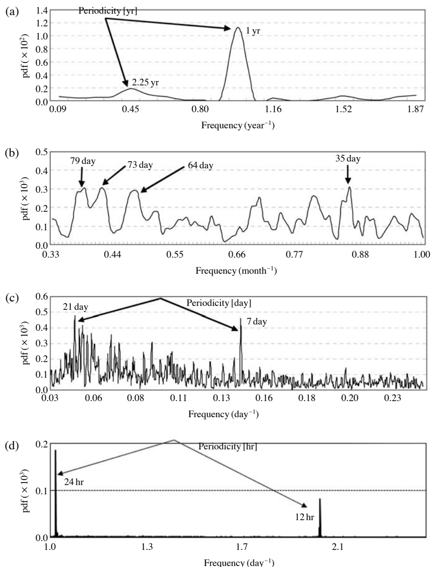
Fig. 3. Power density spectra of PM 10 time series. The frequency dimension is \text{time}^{-1} ( \text{year}^{-1} , \text{month}^{-1} or \text{day}^{-1} ) and the dimension of periodicity is time (year or day).
