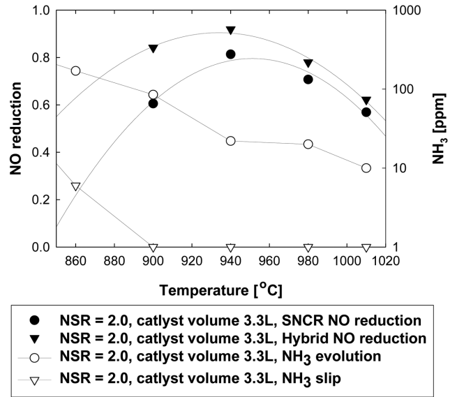
Fig. 9. Effect of reaction temperature on NOx reduction and NH 3 evolution concentration of SNCR and Hybrid SNCR-SCR process (Note : NSR=2.0, SV=18,000~41,000 h -1 ).
