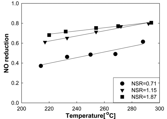
Fig. 5. Effect of reaction temperature on NO reduction of SCR process with a variation of NSR (Note : SV=22,000 h -1 ).
