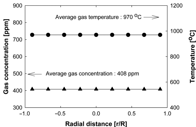
Fig. 2. Radial profile of gas concentration and temperature at nozzle injection point.
