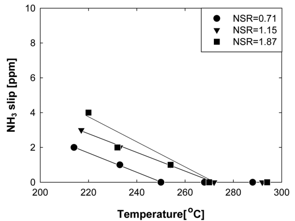
Fig. 6. Effect of reaction temperature on NH 3 slip of SCR process (Note : SV=22,000 h -1 ).
