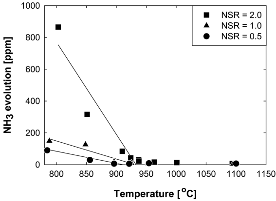
Fig. 4. Effect of reaction temperature on the NH 3 evolution concentration of SNCR process with a variation of NSR.
