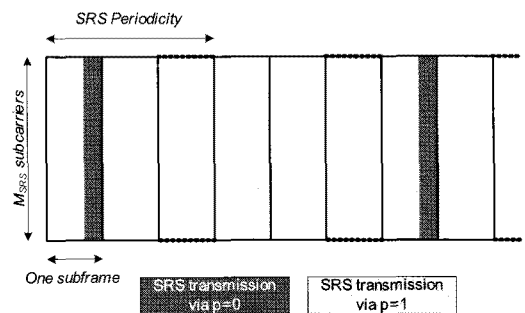
Fig. 3. Wideband SRS transmission (P=2)
