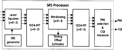
Fig. 4. SRS processing using four receive antennas
