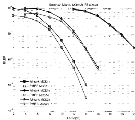
Fig. 6. Performance of MIMO DFT-SOFDMA due to precoding selection with high mobility (16-QAM, 64-QAM)
