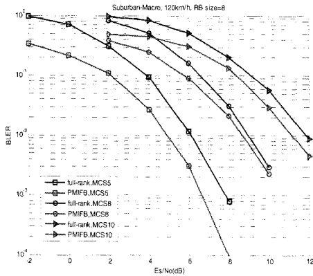
Fig. 5. Performance of MIMO DFT-SOFDMA due to precoding selection with high mobility(QPSK)
