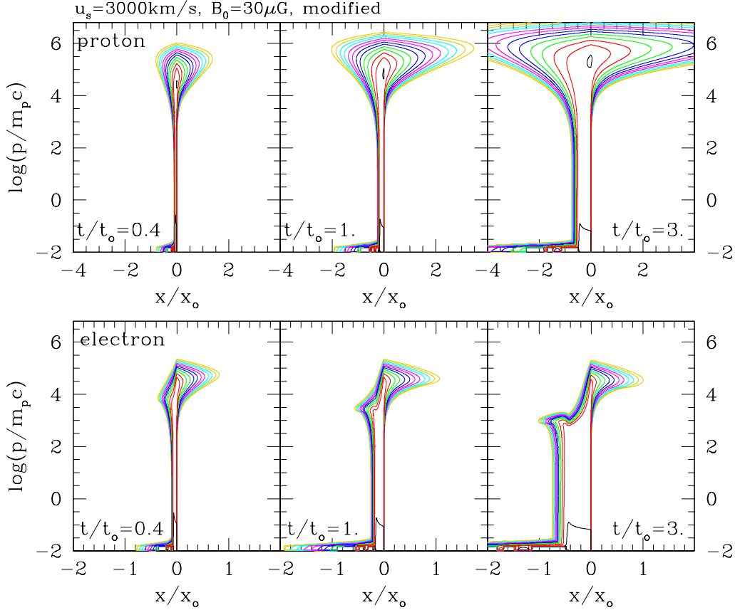
Fig. 5. — Proton and electron distribution functions, g_p(x, p) and g_e(x, p) , in the phase-space at t/t_0 = 0.4, 1, 3 for the CR modified case shown in the bottom panels of Fig. 4. At each contour level, the value of g increases by a factor of 10. Note that the spatial span of the proton distribution shown here is [-4, +4] , while that of the electron distribution is [-2, +2] . (A color version of this figure is available in the online journal.)
