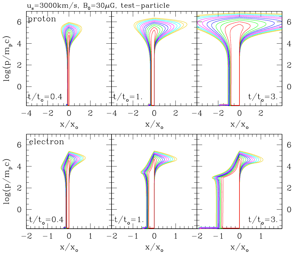
Fig. 3. — Proton and electron distribution function, g_p(x, p) and g_e(x, p) , in the phase-space at t/t_0 = 0.4, 1, 3 for the test-particle case shown in Fig. 2. At each contour level, the value of g increases by a factor of 10. Note that the spatial span of the proton distribution shown here is [-4, +4] , while that of the electron distribution is [-2, +2] . (A color version of this figure is available in the online journal.)
