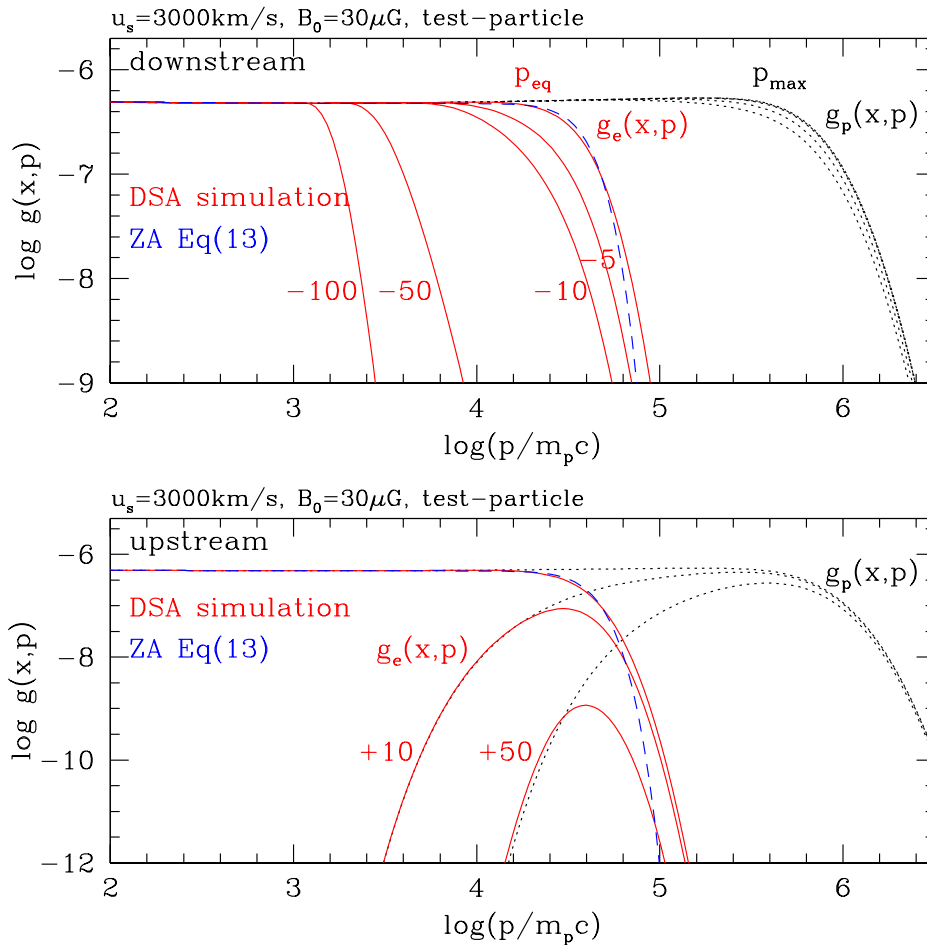
Fig. 2. — Particle spectra from the test-particle DSA simulation for u_s = 3000 \text{ km s}^{-1} , B_0 = 30 \mu\text{G} . Top: Proton spectrum g_p(x, p) (dotted lines) and electron spectrum g_e(x, p) (solid lines) at 5 different locations downstream of the shock at t/t_0 = 5 are shown. The curves for the electron spectrum are labeled with the distance downstream from the shock in the number of grid zones (-100, -50, -10, -5, 0). Note that the cooling length, l_{\text{eq}} , for electrons with p_{\text{eq}} , corresponds to 6.15 grid zones in the simulation. The dashed line shows the analytic form for the electron spectrum at the shock (Eq. [18]) suggested by Zirakashvili & Aharonian (2007). Bottom: Same as above except the spectra at two locations (+10 and +50 grid zones) upstream of the shock are shown along with the spectra at the shock position. (A color version of this figure is available in the online journal.)
