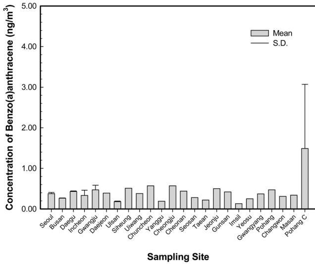
Figure 12. Variation of Benzo(a)anthracene concentration as a function of investigation region in Korea.
