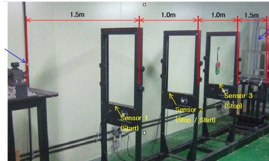
Fig. 1 Anti-bullet testing facility at Samyang ComTech.
