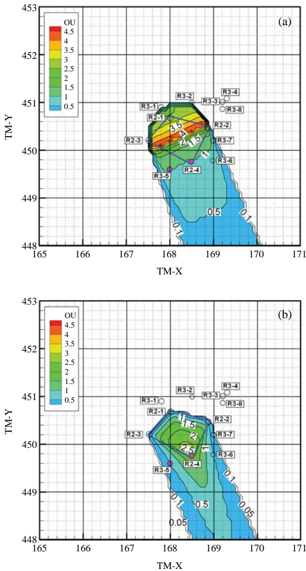
Fig. 3. Odor Unit contour of selected day (Case 6, 7: Time: 2006-08-07-20:00). (a) CALPUFF, (b) AERMOD
