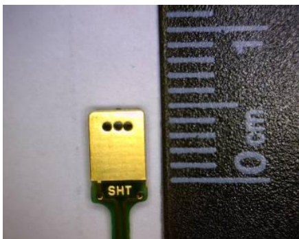
FIGURE 5 H/T SENSOR
