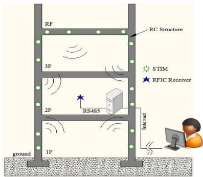
FIGURE 1 APPLYING STIMSTO REMOTE MONITORING OF EXTERIOR WALLS
