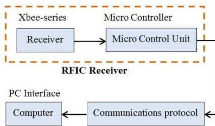
FIGURE 4 WORK PROCESS AT RF RECEIVING END
