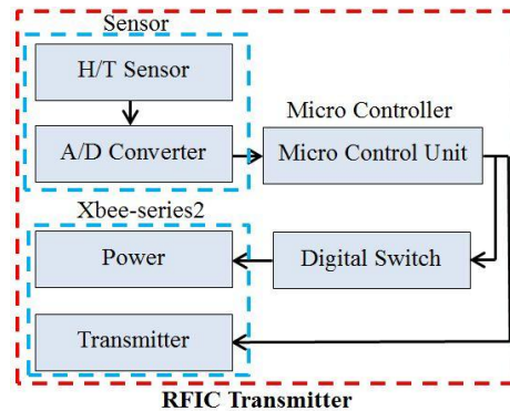
FIGURE 3 WORK PROCESS AT THE RF SENDING END
