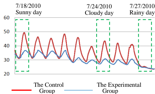
FIGURE 10 TEMPERATURE MEASUREMENTS OF THE INSULATION MATERIAL
