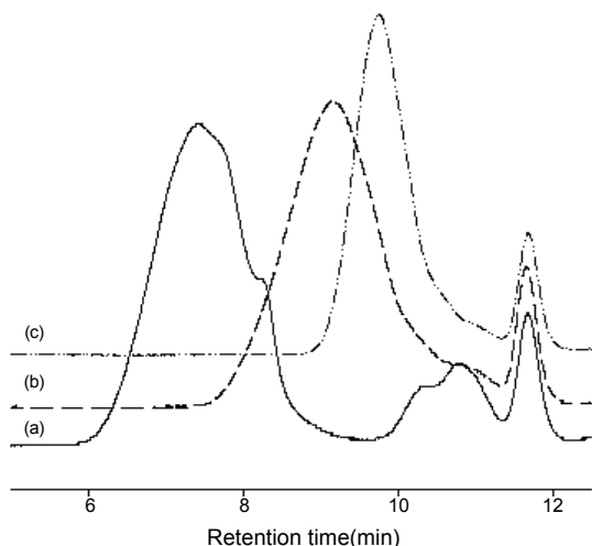
Figure 8. GPC profile of HMWSA(a); LMWSAs treated for 0.5 hr(b); 3.0 hr(c). (2 wt% in reactant concentration and 3 wt% H 2 O 2 at 50 °C with ultrasound).
