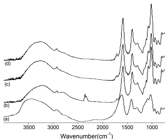
Figure 1. FTIR spectra of HMWSA (a); LMWSAs treated with 2 wt% \text{H}_2\text{O}_2 (b); 6 wt% \text{H}_2\text{O}_2 (c); 15 wt% \text{H}_2\text{O}_2 (d). (2 wt% in reactant concentration; at 50 °C for 30 min with ultrasound).
