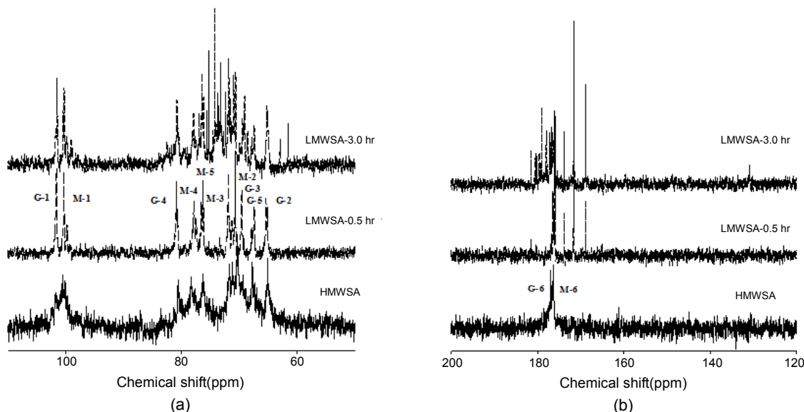
Figure 5. 13 C NMR spectra of alginates in C1–C5 region (a); C6 region (b). G–i and M–i are the different carbon number of guluronate and mannuronate units in sodium alginate (2 wt% in reactant concentration and 3 wt% H 2 O 2 at 50 °C with ultrasound).
