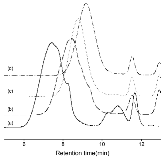
Figure 7. GPC profile of HMWSA(a); LMWSAs treated at 30 °C (b); 40 °C (c); 50 °C (d). (2 wt% in reactant concentration and 3 wt% H 2 O 2 for 30 min with ultrasound).
