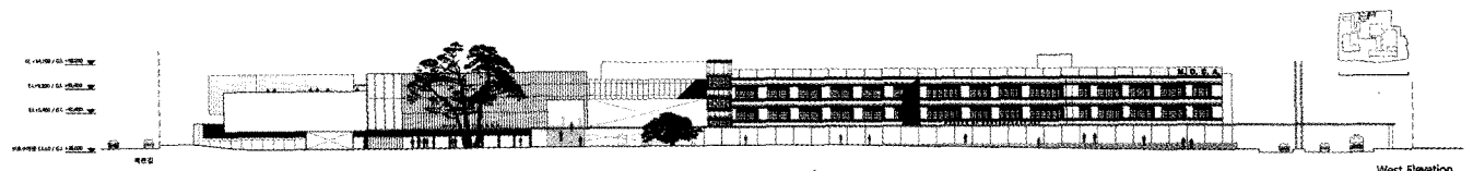
West Elevation
