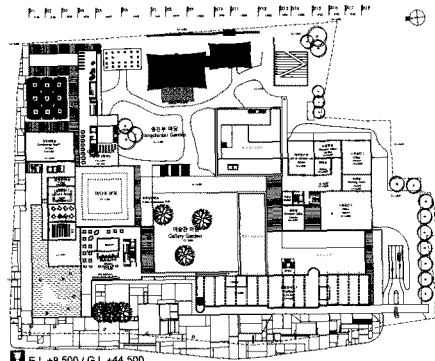
8 EL. +8,500 / G.L. +44,500 (8층 850 Level) scale 1:500
