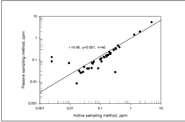
Fig 1. The relationship between passive and active sampling method( r=0.95 , p<0.001 , n=40 ).
