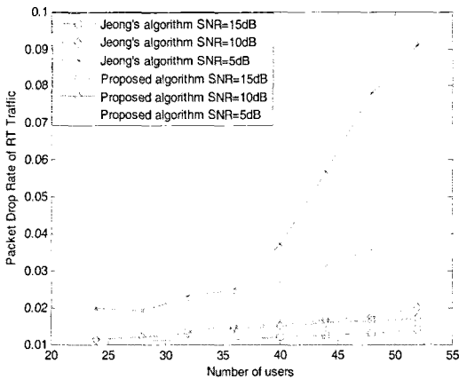
Fig. 3. Packet drop rate of RT traffic according to the number of users
