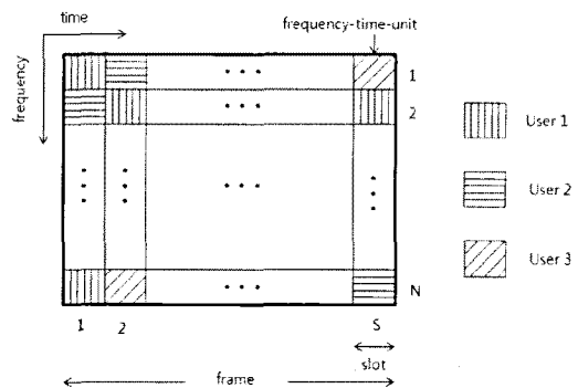
Fig. 1. OFDMA system in frequency-time axis
