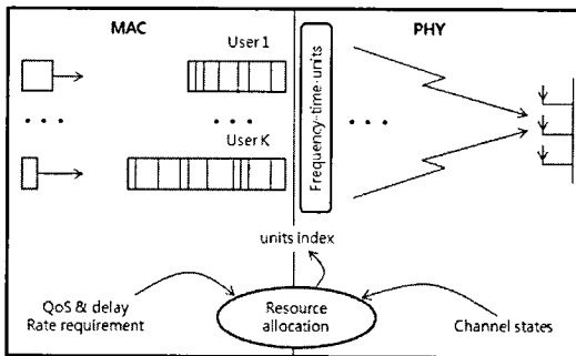
Fig. 2. Procedure of cross-layer resource allocation algorithm
