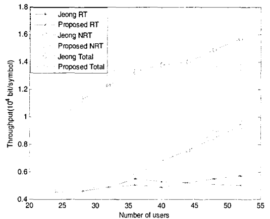
Fig. 4. Throughput according to the number of users
