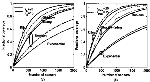
Fig. 3. Fractional coverage analysis: (a) Different r_b with constant M=1000 \times 1000 m^2 , r_{max} = 30m and \beta=0.1 , and (b) Different r_{max} with constant M=1000 \times 1000 m^2 , r_b = 20m and \beta=0.1
