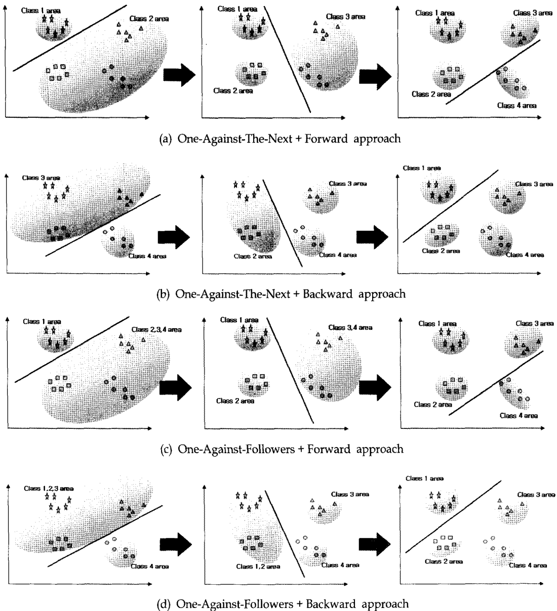
<Figure 2> Differences Among Four Types of the Ordinal Multiclass SVMs: Graphical Presentation
