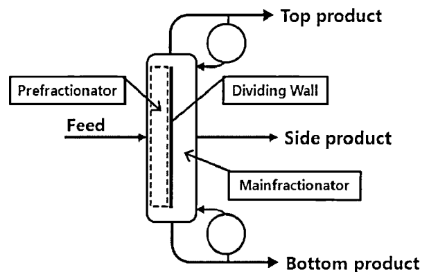
Figure 3. Structure of the typical divided wall column.
