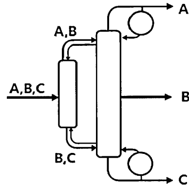
Figure 2. Structure of the typical Petlyuk column.
