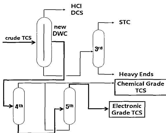
Figure 6. Application of the divided-wall column to the TCS refining process.
