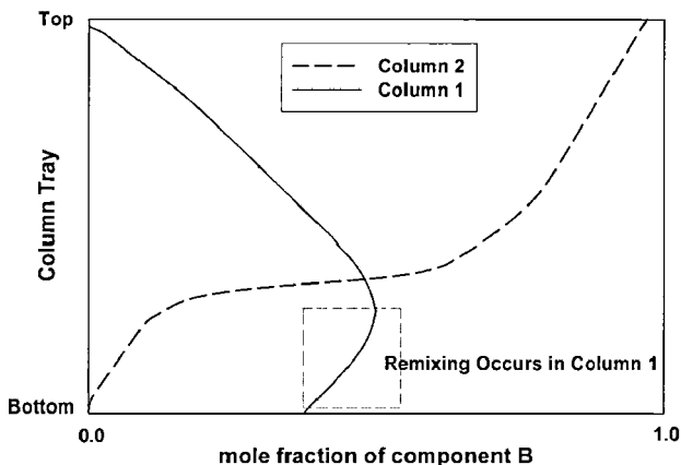
Figure 1. Remixing in a conventional distillation column.
