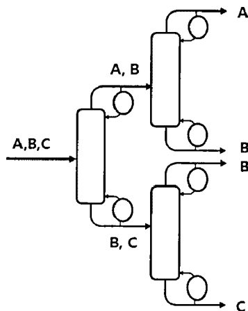
Figure 8. A schematic diagram of the sloppy column configuration for the DWC structure design.
