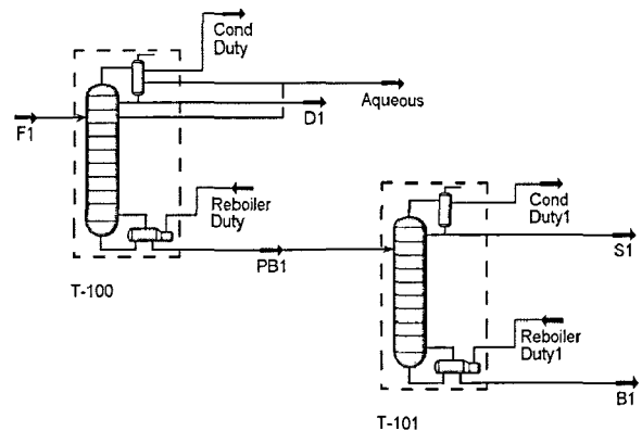
Figure 1. Process diagram of the conventional distillation system.
