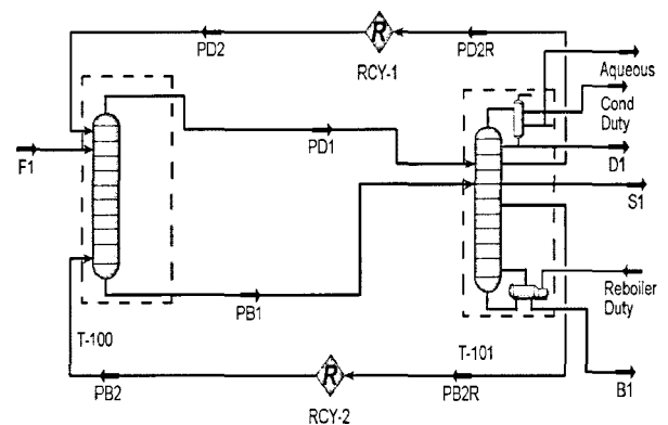
Figure 2. Process diagram of the thermally-coupled distillation system.
