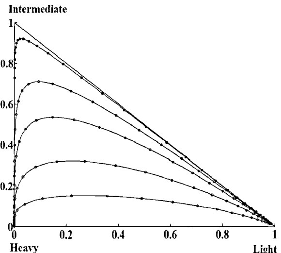
Figure 3. Residue curves of a typical ternary system.
