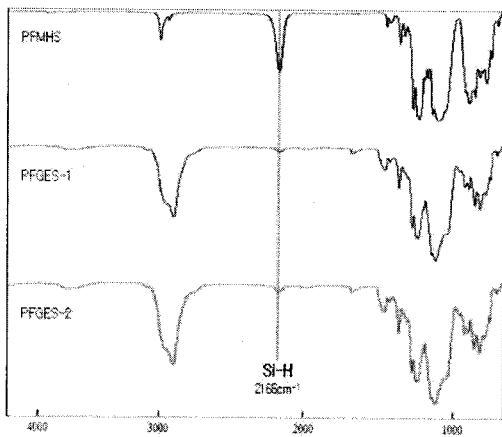
Fig. 2. FT-IR spectra of PFMHS and PFGES-1, PFGES-2
