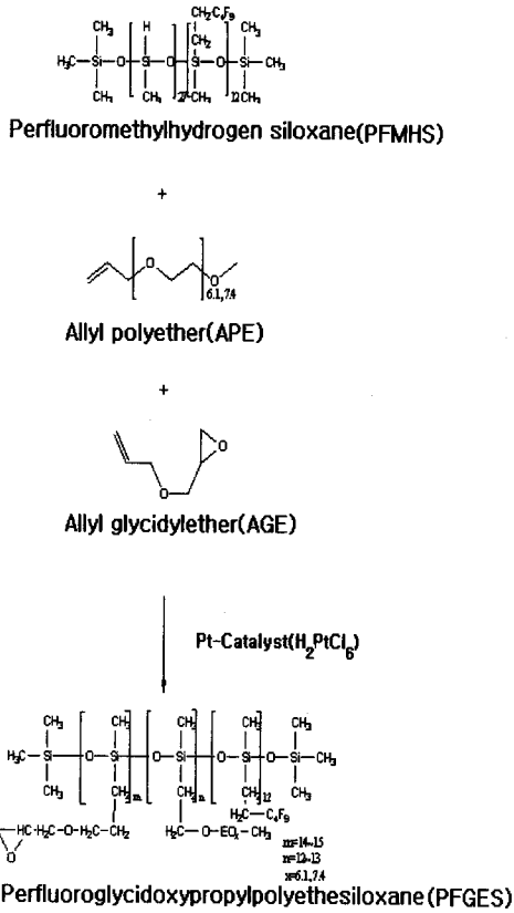
Scheme 1. Synthesis of epoxy functionalized fluoro-silicone surfactant.
