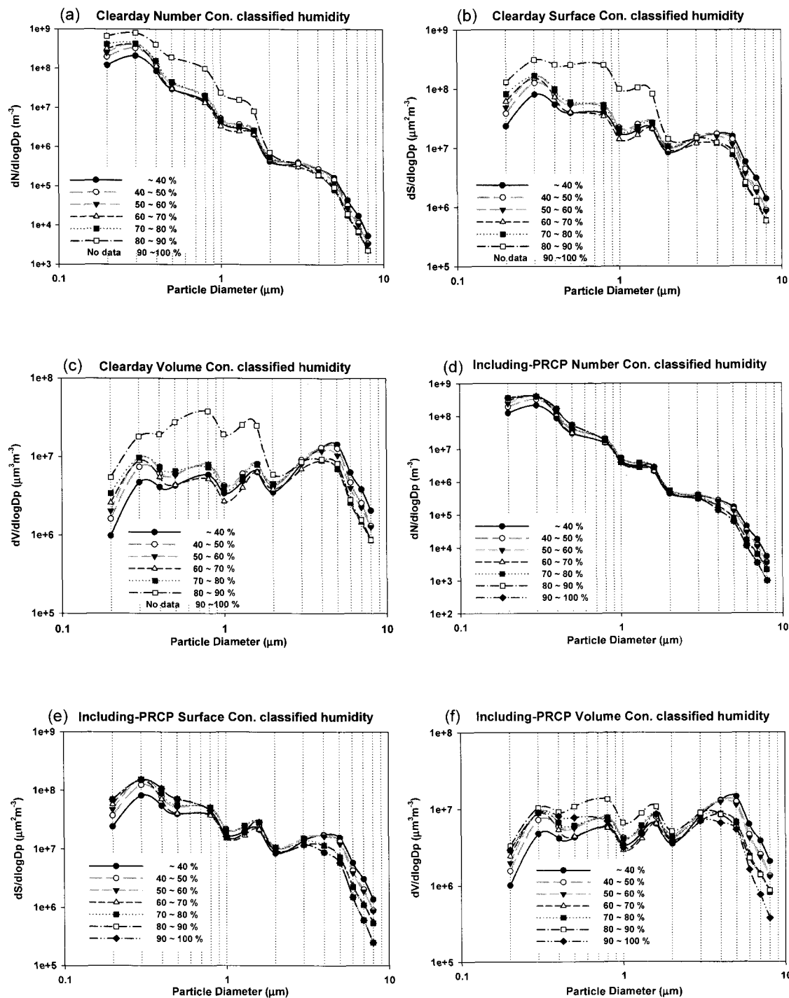
Fig. 6. Aerosol size distributions as a function of the classified humidity.
