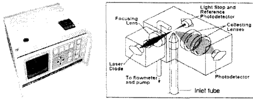
Fig. 2. Schematic of the Laser Particle Counter.
