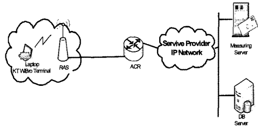
Fig. 1. Mobile WiMAX network architecture for data collection
