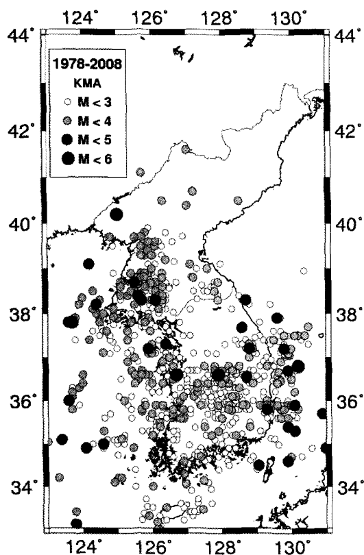
Fig. 2. Epicentral Distribution of the Instrumental Earthquakes (1978-2008, KMA[10])
