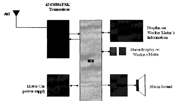
Fig. 2. Configuration of the on-board terminal.
