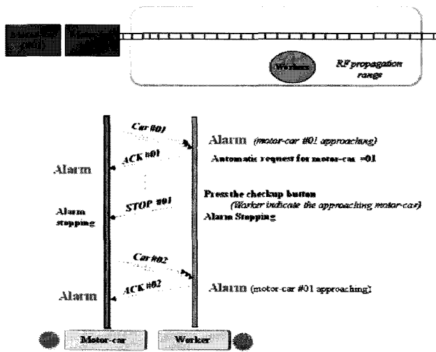
Fig. 4. Basic alarm operation mechanism.
