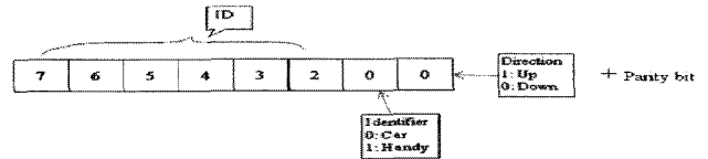
(b) Structure of the transmission frame for worker terminal → On-board terminal
