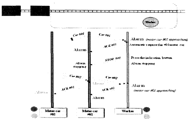
Fig. 6. Alarm operation mechanism the motor-carworker and between motor-scars.
