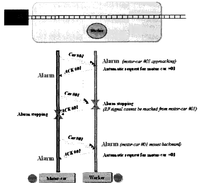
Fig. 5. Alarm mechanism when the motor-car moves backward after leaving its propagation area.
