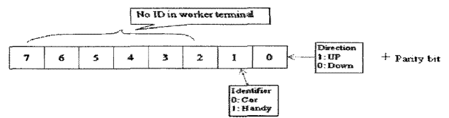
(a) Structure of the transmission frame for on-board terminal → Worker terminal
