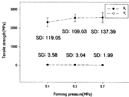
Fig. 5 Tensile strength according to the forming pressure.
