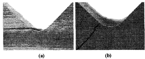
Fig. 14 Typical shear failures of ILS test specimens of UD carbon/poxy laminate: (a) the 1-3 shear plane, (b) the 2-3 shear plane.
