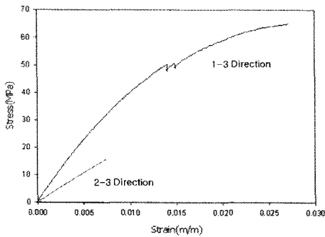
Fig. 11 Stress-strain curves of out-of-plane shear tests.
