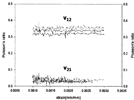
Fig. 6 Poisson's ratio from the tensile tests.
