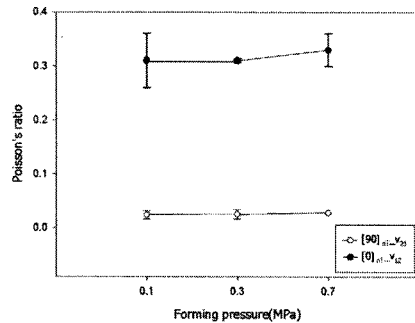
Fig. 7 Poisson's ratio according to the forming pressure.
