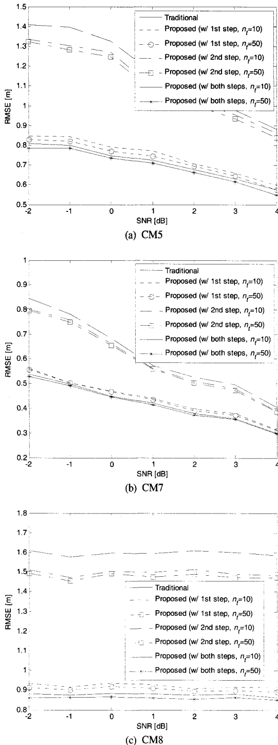
Fig. 4. The location RMSE comparison of the proposed scheme and the traditional TDoA localization in IEEE.802.15.4a channel models.
