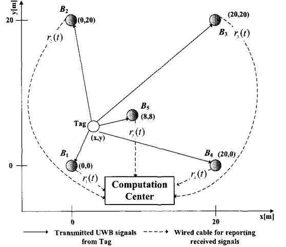
Fig. 1. System model for UWB localization.
