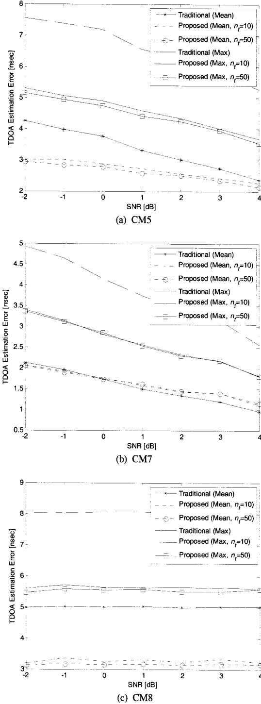
Fig. 3. The estimation performance of the TDoA parameters in IEEE 802.15.4a channel models.
