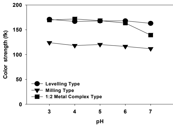
Fig. 6. Color strength of regular type nylon dyed at different pH conditions (2%o.w.f.).
