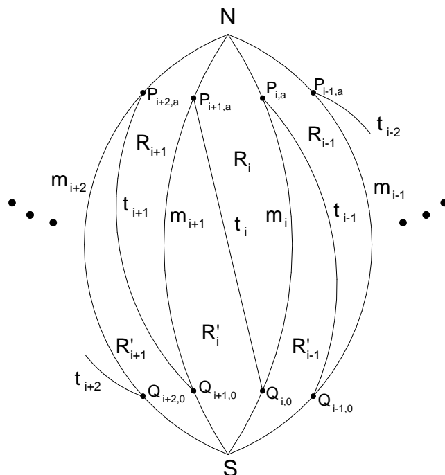
FIGURE 2. Polyhedral description of generalized Dunwoody manifolds
