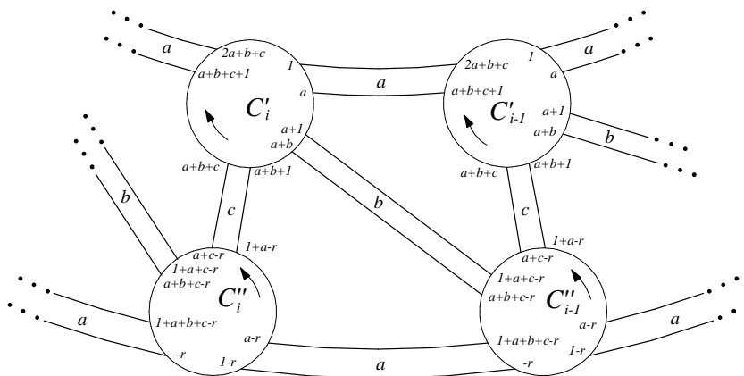
FIGURE 1. A Dunwoody diagram
