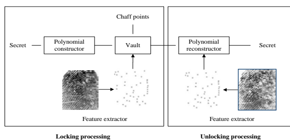
Fig. 4. Fuzzy fingerprint vault block diagram
