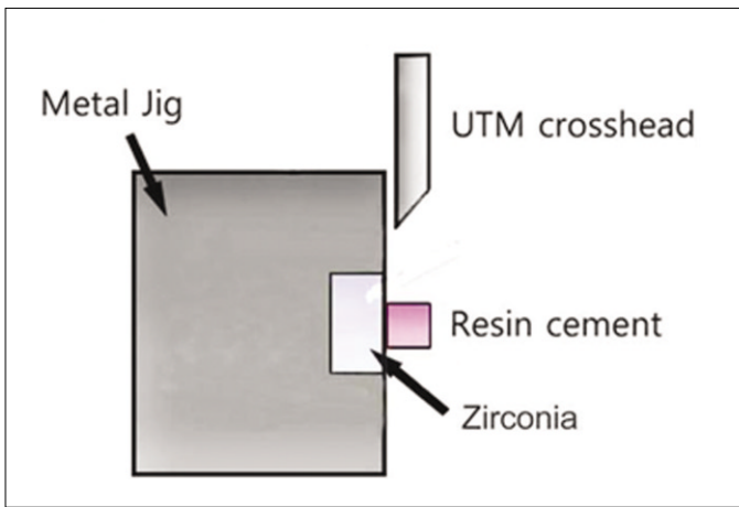
Fig. 4. Schematic diagram of shear bond strength testing.
