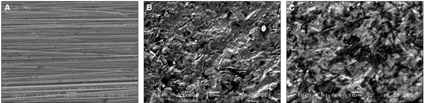
Fig. 9. SEM pictures of Zirconia ceramic (magnification × 1,000).
