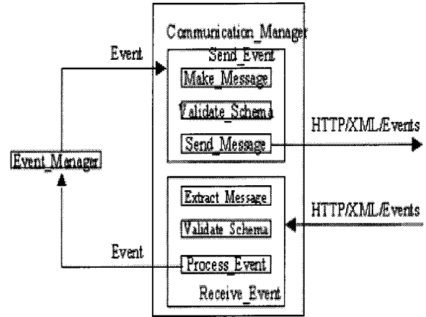
Fig. 5. Communication Manager
