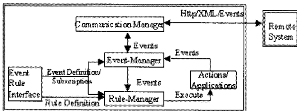
Fig.4. Overall Architecture of Active Rule Component
