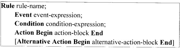
Fig. 3. Active Rule Structure
