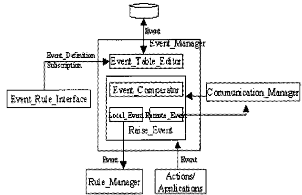
Fig. 6. Event Manager
