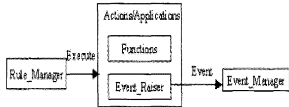
Fig. 9. Actions/Applications
