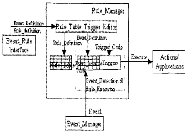
Fig. 7. Rule Manager
