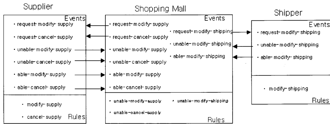
Fig. 10. Events and Rules for Intimate Cooperation
