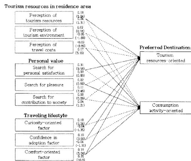
Fig. 2. Path Analysis Model
