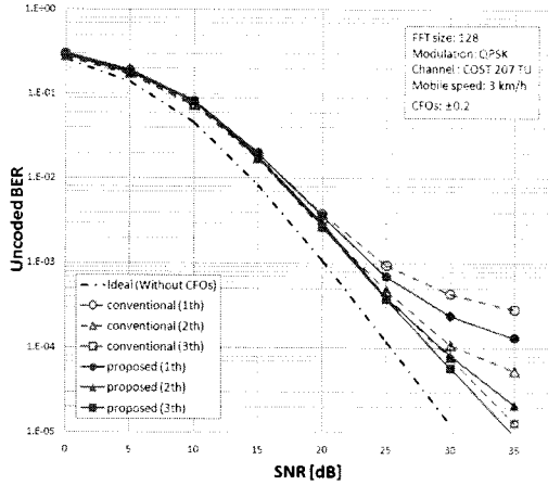
(a) QPSK
