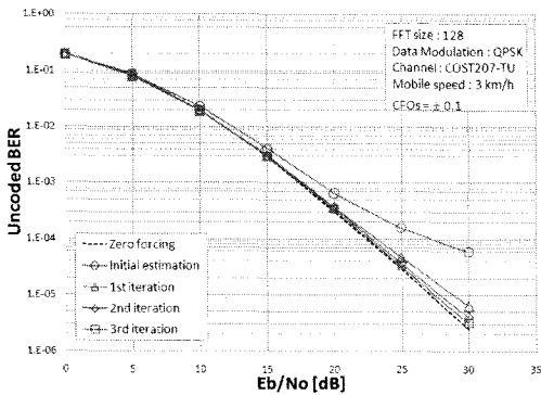
(a) CFOs = ±0.1
