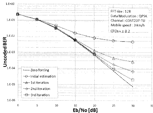
(b) CFOs = ±0.2
