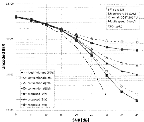
(c) 64-QAM
